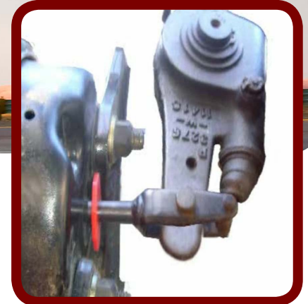
Brake Released
